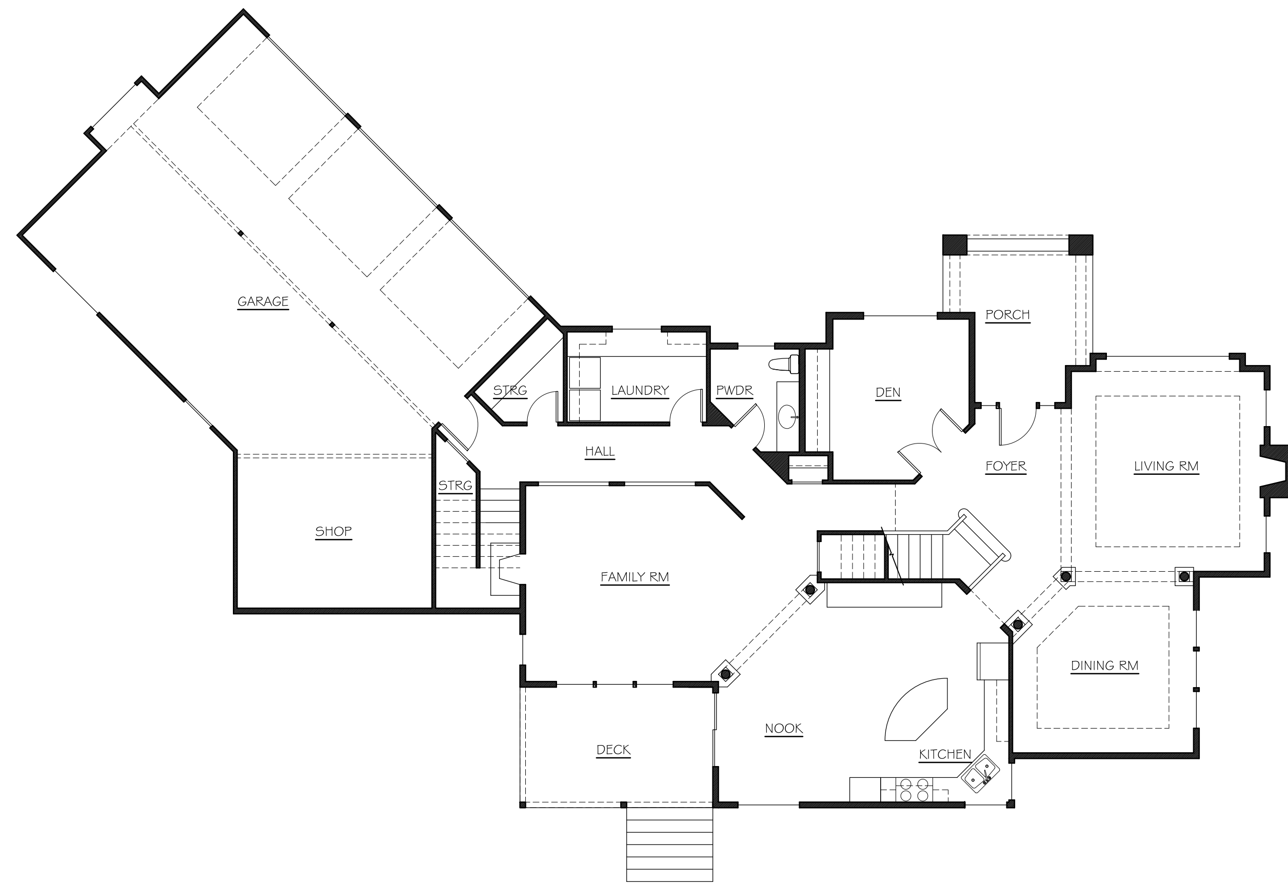
↑ MAIN FLOOR PLAN - BEFORE
